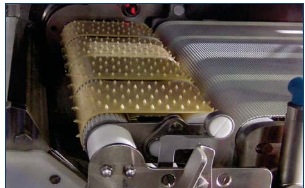
SMW welded closed and used as a narrow flat belt
