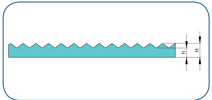
IRT Belt Thickness Diagram
