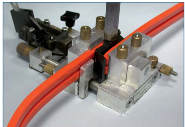
Easy Overlap Schweißwerkzeug
