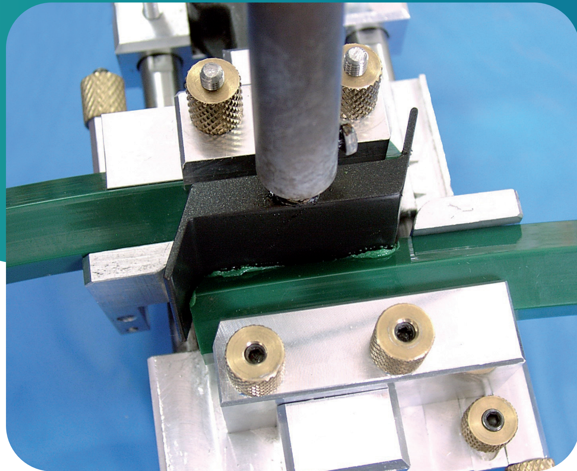
Easy Overlap Welder (EZOL) for Reinforced profiles
