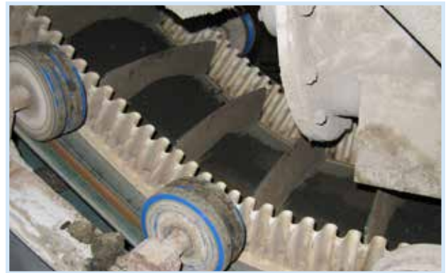
FRG-3 with thermo welded sidewalls and flights: CHEMICAL POWDER (RECYCLED SEWAGE)
