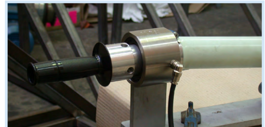
Sleeve mounting
